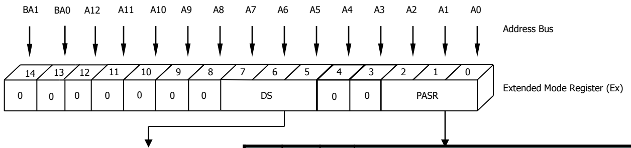
Figure5: Extended Mode Register
