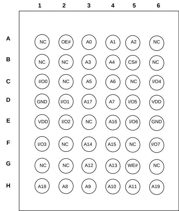
48-Pin mini BGA (6mm x 8mm), 1 CS
