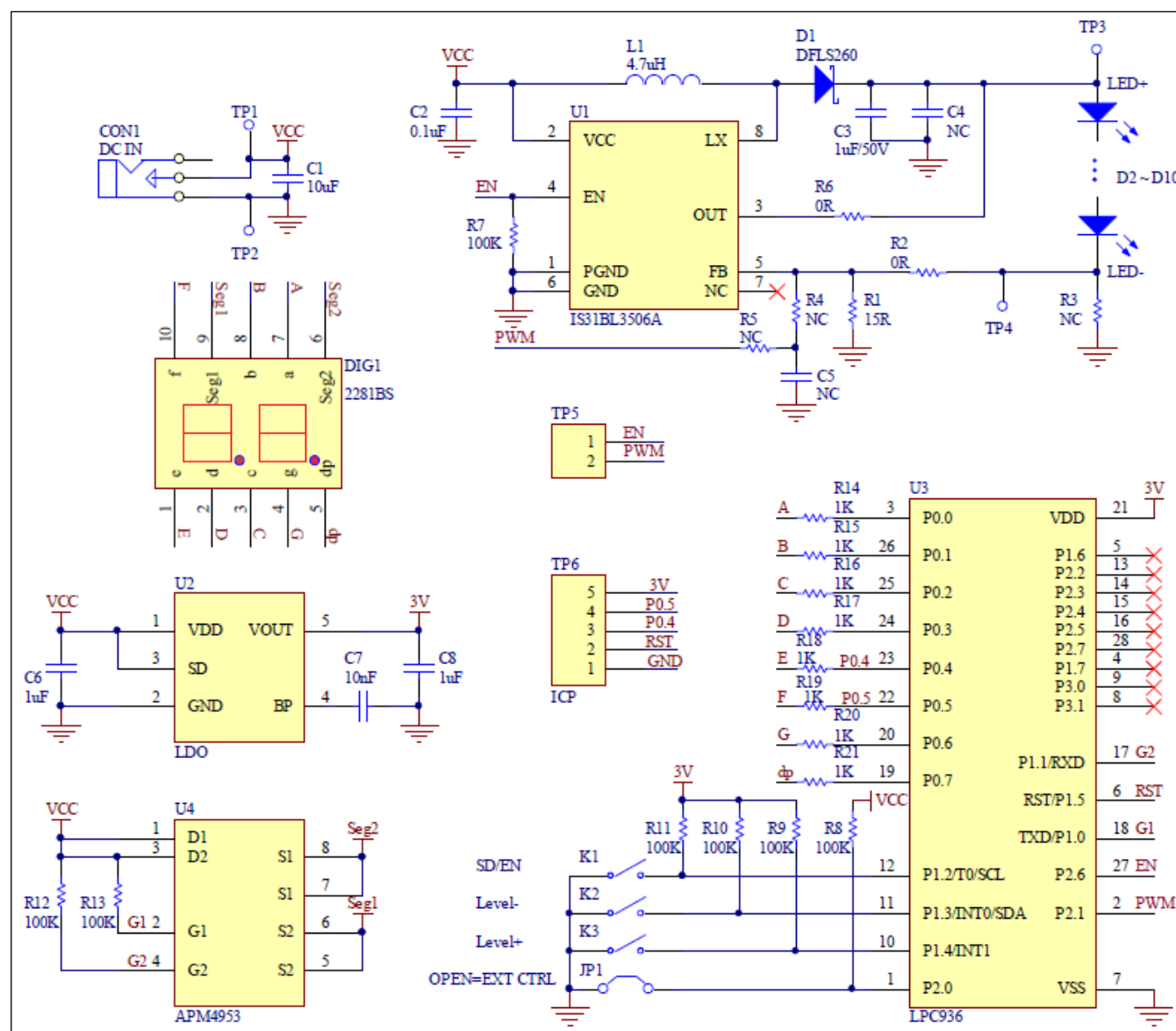
Figure 2: IS31BL3506A Application Schematic
