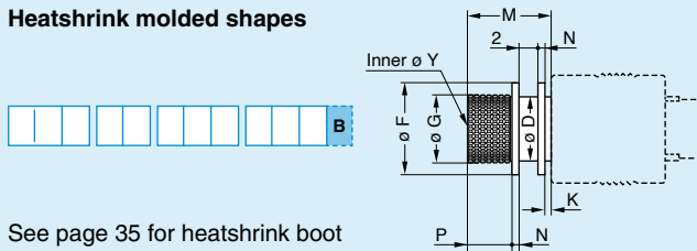
Heatshrink molded shapes
