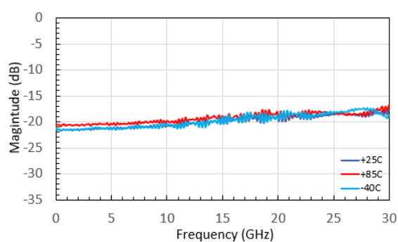
Output Return Loss, over Temperature
