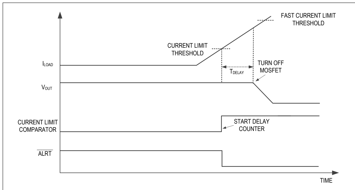
Figure 2. Overcurrent Event
