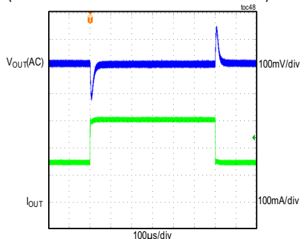
MAXM17906 LOAD TRANSIENT RESPONSE V_{IN} = 12V , ADJUSTABLE V_{OUT} = 5V , PWM MODE (LOAD CURRENT STEPPED FROM 150mA TO 300mA)
