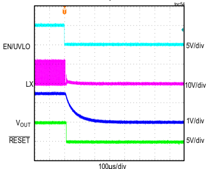
MAXM17906 SHUTDOWN THROUGH ENABLE V_{IN} = 12V , ADJUSTABLE V_{OUT} = 1.5V , FULL LOAD, PWM MODE
