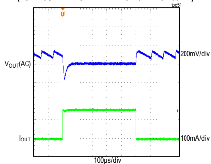
MAXM17905 LOAD TRANSIENT RESPONSE V_{IN} = 12V , FIXED V_{OUT} = 5V , PFM MODE (LOAD CURRENT STEPPED FROM 5mA TO 150mA)
