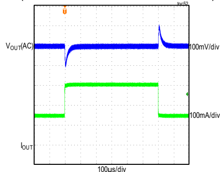
MAXM17905 LOAD TRANSIENT RESPONSE V_{IN} = 12V , FIXED V_{OUT} = 5V , PWM MODE (LOAD CURRENT STEPPED FROM 150mA TO 300mA)
