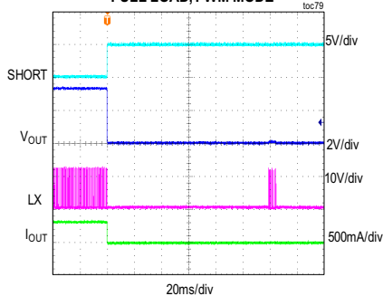
MAXM17906 OUTPUT SHORT IN STEADY STATE V_{IN} = 12V , ADJUSTABLE V_{OUT} = 3.3V , FULL LOAD, PWM MODE
