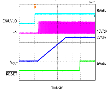
MAXM17905 STARTUP THROUGH ENABLE V_{IN} = 12V , FIXED V_{OUT} = 5V , FULL LOAD, PWM MODE
