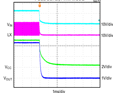
MAXM17906 SHUTDOWN THROUGH V_{IN} V_{IN} = 12V , ADJUSTABLE V_{OUT} = 3.3V , FULL LOAD, PWM MODE
