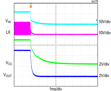
MAXM17905 SHUTDOWN THROUGH V_{IN} V_{IN} = 12V , FIXED V_{OUT} = 5V , FULL LOAD, PWM MODE
