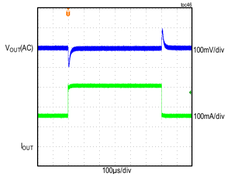
MAXM17906 LOAD TRANSIENT RESPONSE V_{IN}=12V , ADJUSTABLE V_{OUT} = 3.3V , PWM MODE (LOAD CURRENT STEPPED FROM 150mA TO 300mA)
