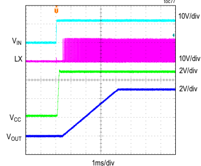
MAXM17905 STARTUP THROUGH V_{IN} V_{IN} = 12V , FIXED V_{OUT} = 5V , FULL LOAD, PWM MODE
