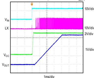
MAXM17906 STARTUP THROUGH V_{IN} V_{IN} = 12V , ADJUSTABLE V_{OUT} = 3.3V , FULL LOAD, PWM MODE
