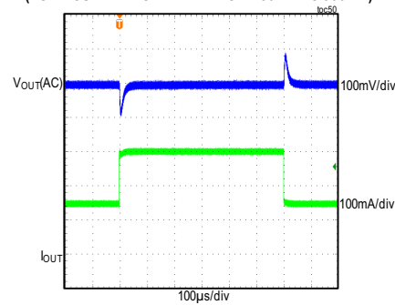
MAXM17904 LOAD TRANSIENT RESPONSE V_{IN} = 12V , FIXED V_{OUT} = 3.3V , PWM MODE (LOAD CURRENT STEPPED FROM 150mA TO 300mA)
