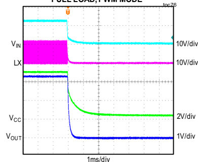
MAXM17904 SHUTDOWN THROUGH V_{IN} V_{IN} = 12V , FIXED V_{OUT} = 3.3V , FULL LOAD, PWM MODE
