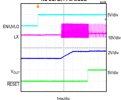
MAXM17904 STARTUP THROUGH ENABLE: 2V PREBIAS V_{IN} = 12V , FIXED V_{OUT} = 3.3V , NO LOAD, PFM MODE
