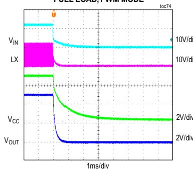
MAXM17906 SHUTDOWN THROUGH V_{IN} V_{IN} = 12V , ADJUSTABLE V_{OUT} = 5V , FULL LOAD, PWM MODE
