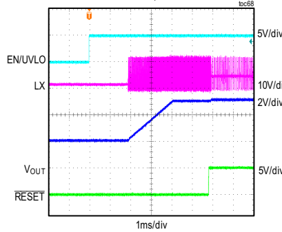
MAXM17905 STARTUP THROUGH ENABLE: 2.5V PREBIAS V_{IN} = 12V , FIXED V_{OUT} = 5V , NO LOAD, PFM MODE
