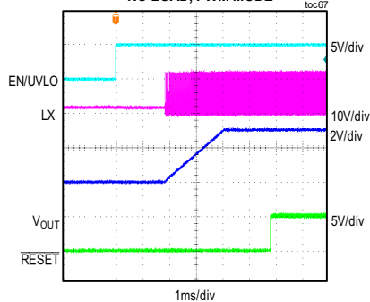
MAXM17905 STARTUP THROUGH ENABLE: 2.5V PREBIAS V_{IN} = 12V , FIXED V_{OUT} = 5V , NO LOAD, PWM MODE
