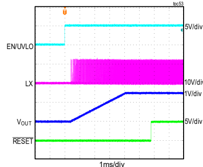
MAXM17906 STARTUP THROUGH ENABLE V_{IN} = 12V , ADJUSTABLE V_{OUT} = 1.5V , FULL LOAD, PWM MODE
