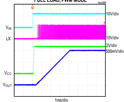
MAXM17906 STARTUP THROUGH V_{IN} V_{IN} = 12V , ADJUSTABLE V_{OUT} = 1.5V , FULL LOAD, PWM MODE
