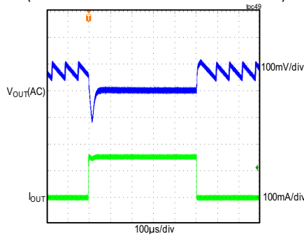
MAXM17904 LOAD TRANSIENT RESPONSE V_{IN} = 12V , FIXED V_{OUT} = 3.3V , PFM MODE (LOAD CURRENT STEPPED FROM 5mA TO 150mA)
