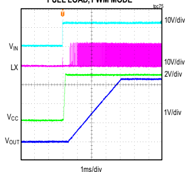
MAXM17904 STARTUP THROUGH V_{IN} V_{IN} = 12V , FIXED V_{OUT} = 3.3V , FULL LOAD, PWM MODE
