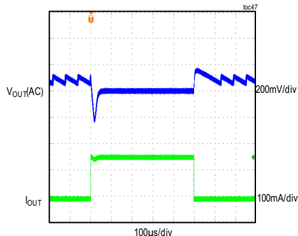
MAXM17906 LOAD TRANSIENT RESPONSE V_{IN} = 12V , ADJUSTABLE V_{OUT} = 5V , PFM MODE (LOAD CURRENT STEPPED FROM 5mA TO 150mA)
