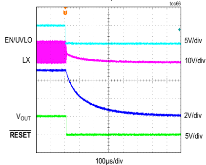
MAXM17905 SHUTDOWN THROUGH ENABLE V_{IN} = 12V , FIXED V_{OUT} = 5V , FULL LOAD, PWM MODE
