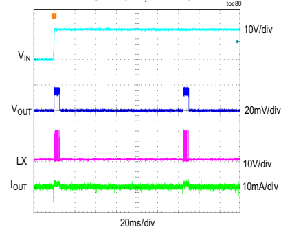
MAXM17906 OUTPUT SHORT DURING STARTUP V_{IN} = 12V , ADJUSTABLE V_{OUT} = 3.3V , FULL LOAD, PWM MODE
