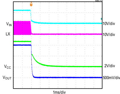
MAXM17906 SHUTDOWN THROUGH V_{IN} V_{IN} = 12V , ADJUSTABLE V_{OUT} = 1.5V , FULL LOAD, PWM MODE
