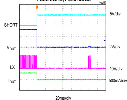
MAXM17904 OUTPUT SHORT IN STEADY STATE V_{IN} = 12V , FIXED V_{OUT} = 3.3V , FULL LOAD, PWM MODE
