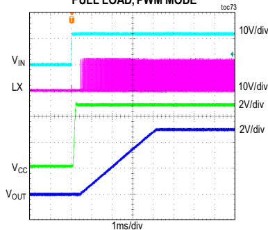
MAXM17906 STARTUP THROUGH V_{IN} V_{IN} = 12V , ADJUSTABLE V_{OUT} = 5V , FULL LOAD, PWM MODE
