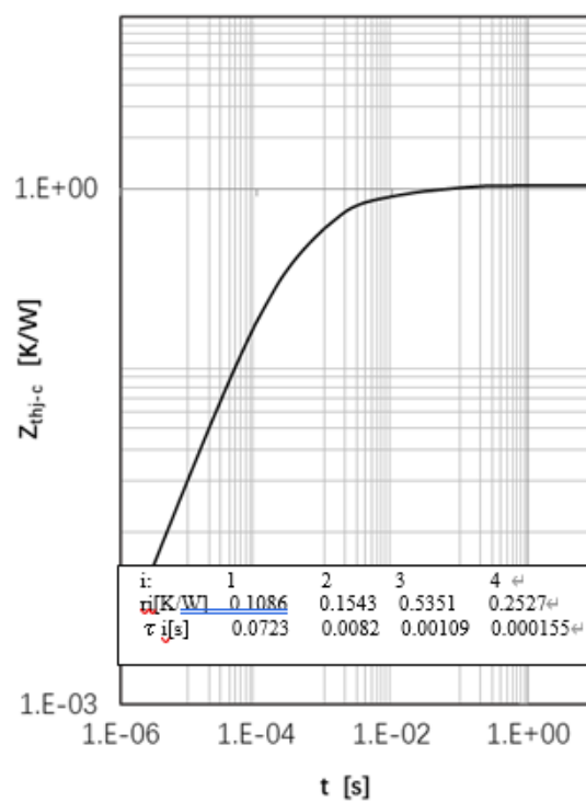
Fig 18. Diode Transient Thermal Impedance
