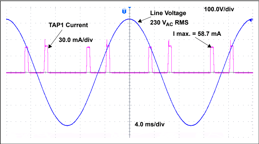
FIGURE C-3: TAP1 Current at 230 V AC Line Input Voltage.
