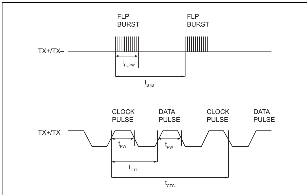
FIGURE 7-11: AUTO-NEGOTIATION TIMING
