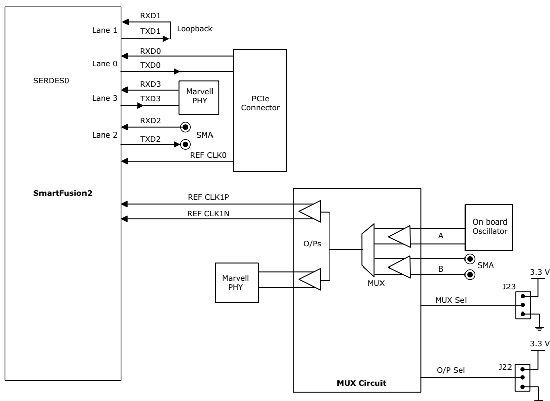
Figure 8 • SERDES0 Interface
