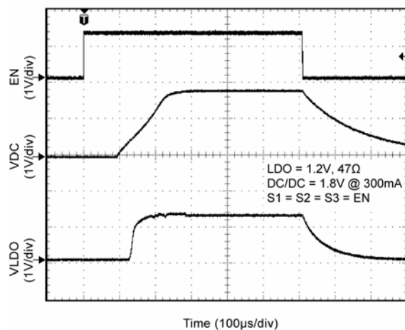
Start-Up Sequence (CDLY = 100pF)
