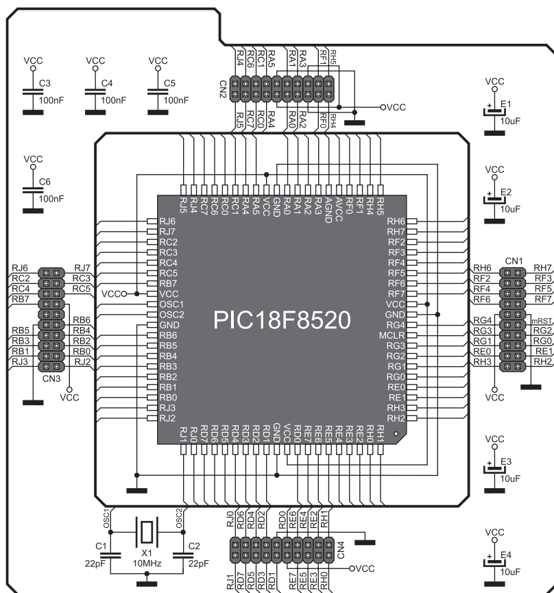
Figure 2: 80-pin MCU card and microcontroller connection schematic
