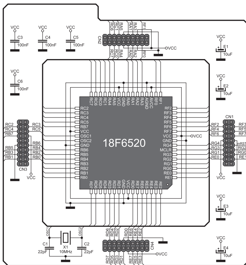
Figure 1: 64-pin MCU card and microcontroller connection schematic
