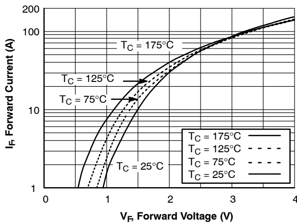
Figure 17. Forward Characteristics
