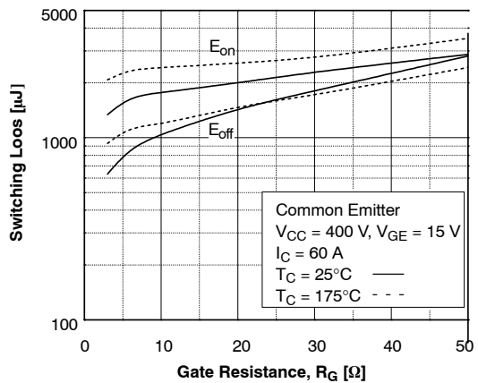
Figure 11. Switching Loos vs. Gate Resistance
