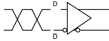
Figure 21. Differential Inputs Driven Differentially
