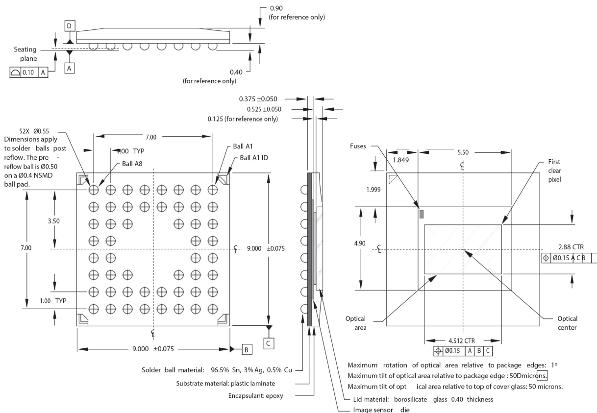
Figure 45: 52-Ball IBGA
