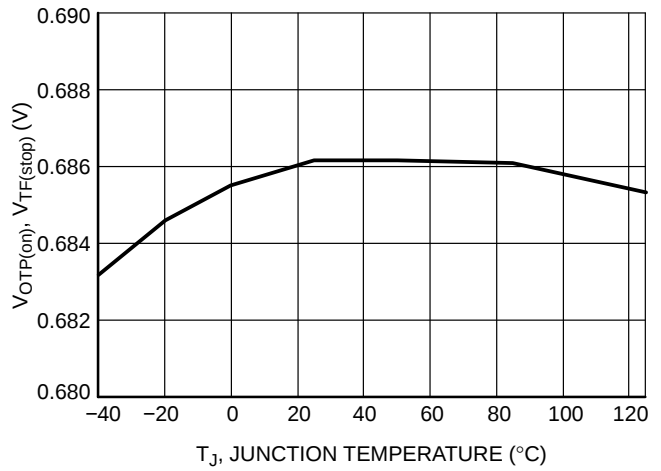
Figure 48. V OTP(on) , V TF(stop) vs. Junction Temperature
