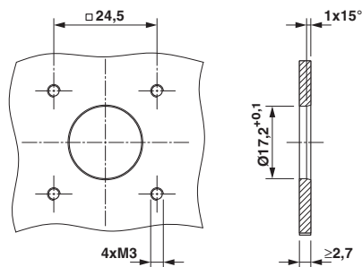
Installation dimensions
