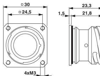
Dimensional drawing
