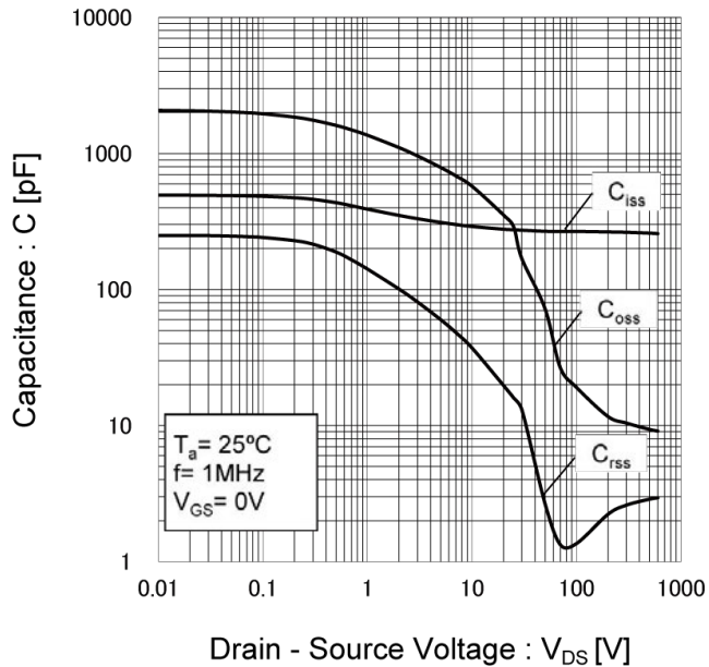
Fig.13 Typical Capacitance vs. Drain - Source Voltage
