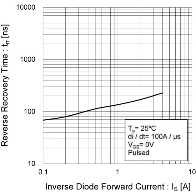
Fig.17 Reverse Recovery Time vs. Inverse Diode Forward Current
