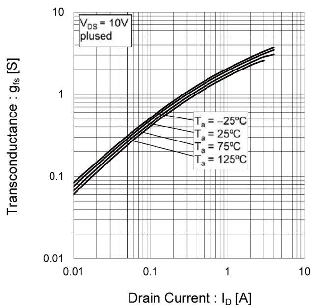
Fig.9 Forward Transfer Admittance vs. Drain Current
