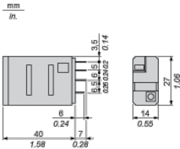
Pin Side View mm in.
