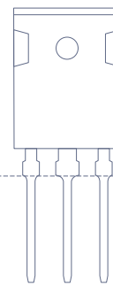
TO-247AD MTO-3P,3PT,3PV
