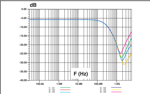
Figure 3. S21 attenuation measurements
