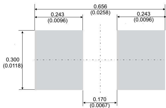
Figure 10. Footprint, dimensions in mm (inches)
