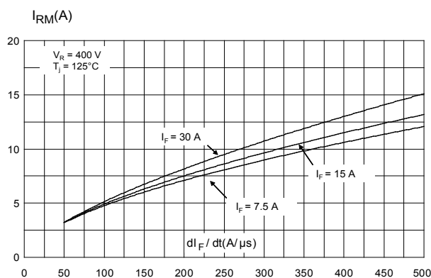
Figure 6. Peak reverse recovery current versus di/dt (typical values)
