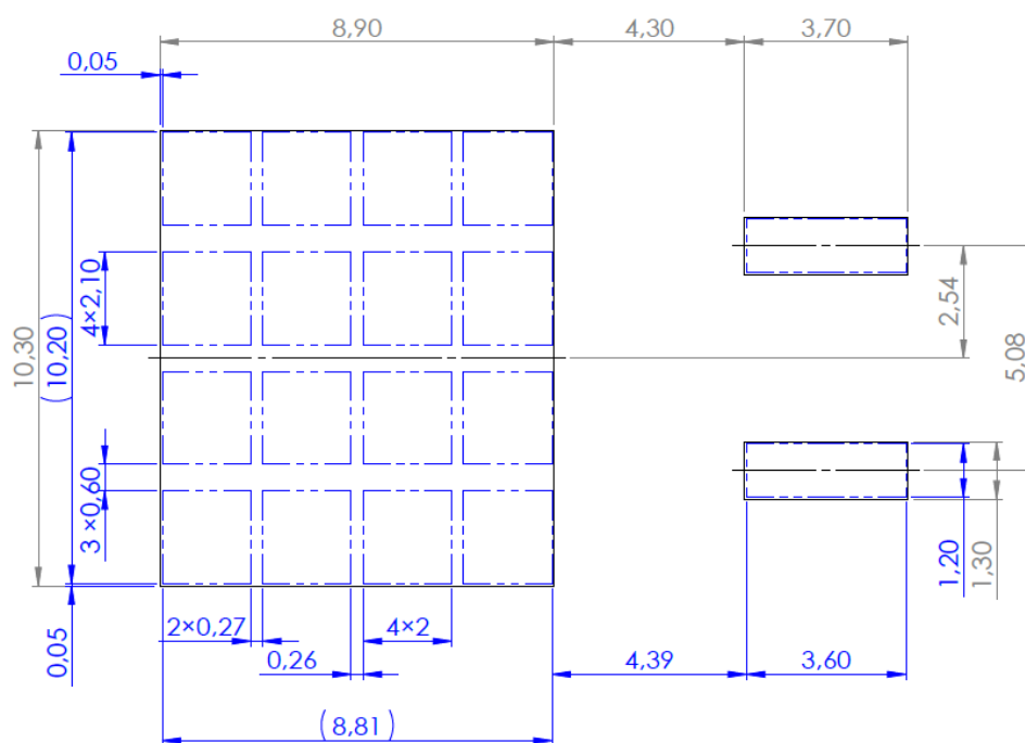
Figure 14. D 2 PAK stencil definitions (dimensions are in mm)
