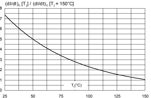
Figure 6. Relative variation of critical rate of decrease of main current versus junction temperature
