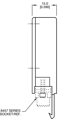
Cover Assembly for 8457 Socket Series, 96-Pin only
