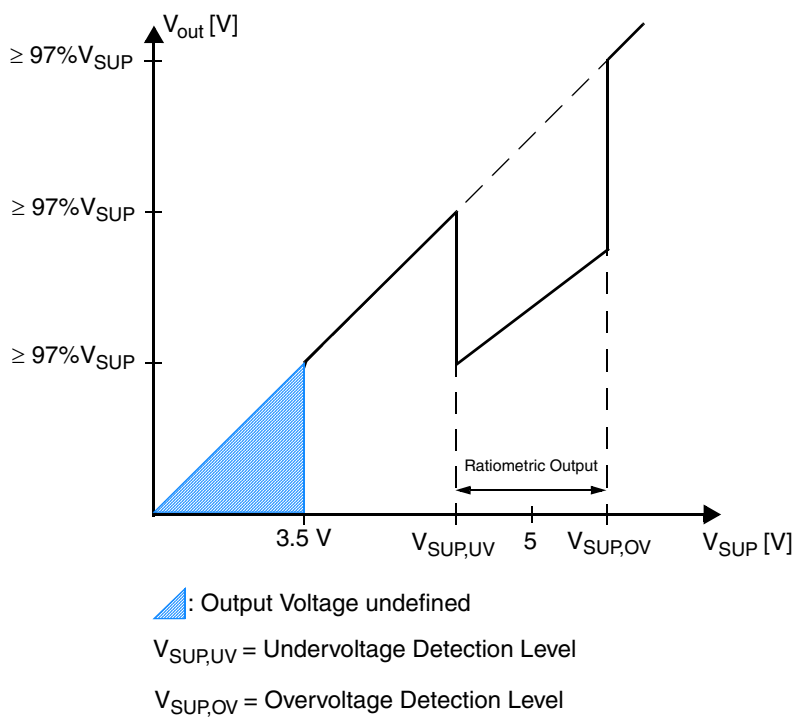
Fig. 4–5: Analog output behavior for different supply voltages
