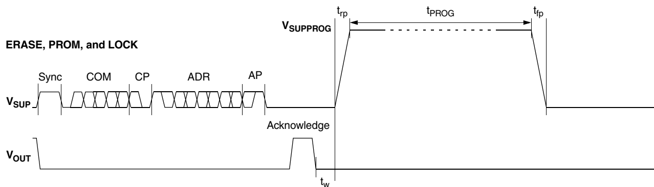
Fig. 6–4: Telegram for coding the EEPROM programming
