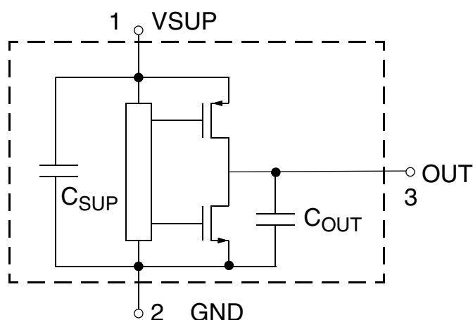
Fig. 4–3: Pin configuration
