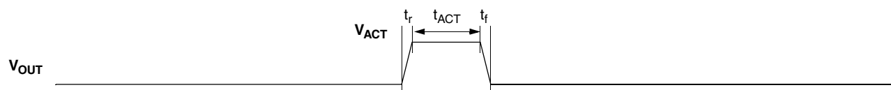
Fig. 6–5: Activate pulse
