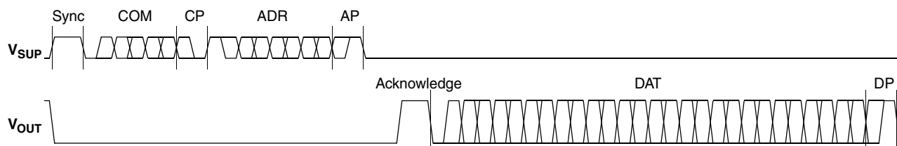
Fig. 6–3: Telegram for coding a Read command
