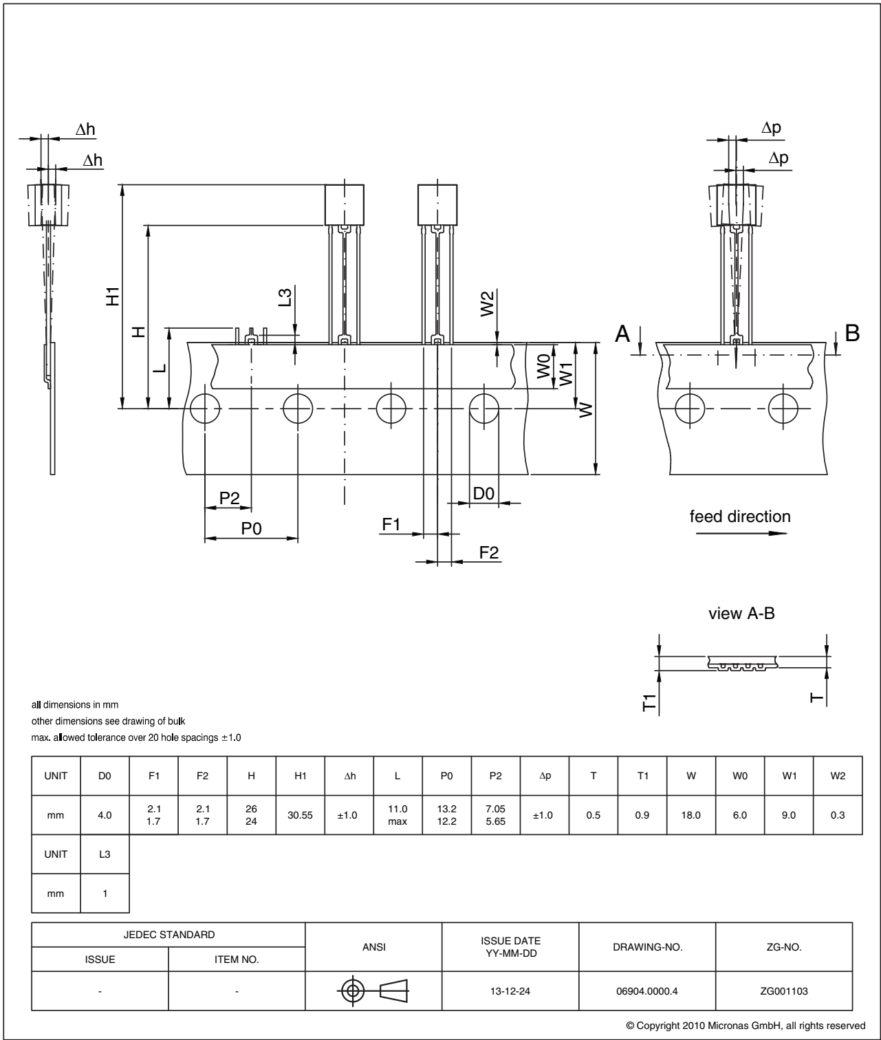
Fig. 4-2: TO92UP-2: Dimensions ammopack inline, not spread
