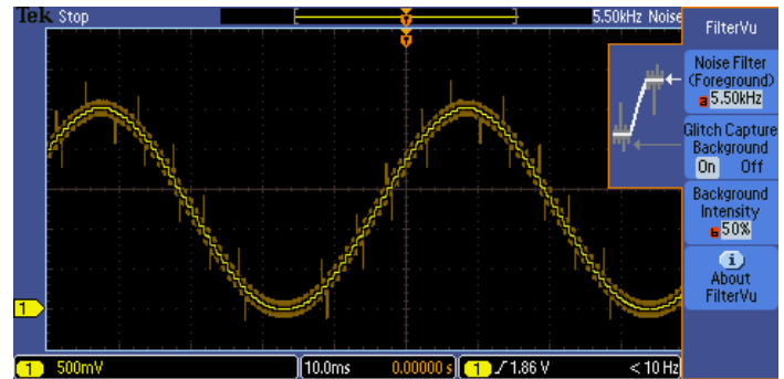
Output of DAC Signal - Notice how FilterVu™ clearly shows the noise-free steps of the DAC in the foreground trace (yellow) which has removed all frequencies above 5.5 kHz. FilterVu also captures and displays high-frequency glitches up to the full bandwidth of the oscilloscope in the background trace (orange).
