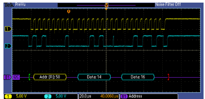
Triggering on a specific data packet going across an I 2 C bus. The yellow waveform is clock and the blue waveform is data. A bus waveform provides decoded packet content including Start, Address, Read/Write, Data, and Stop.
