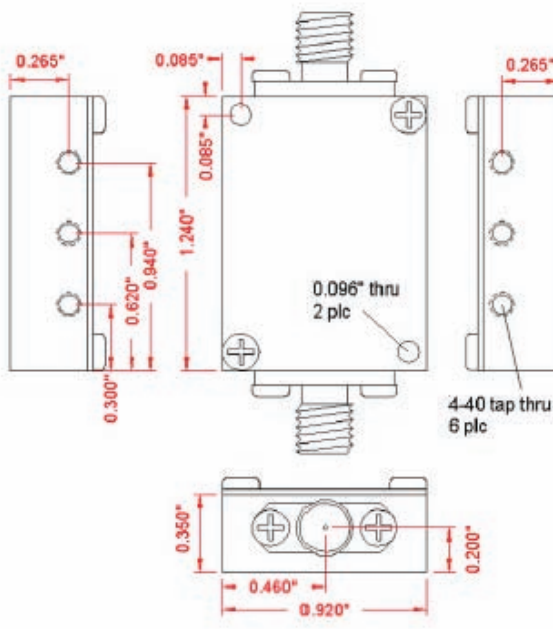
OUTLINE DRAWING
