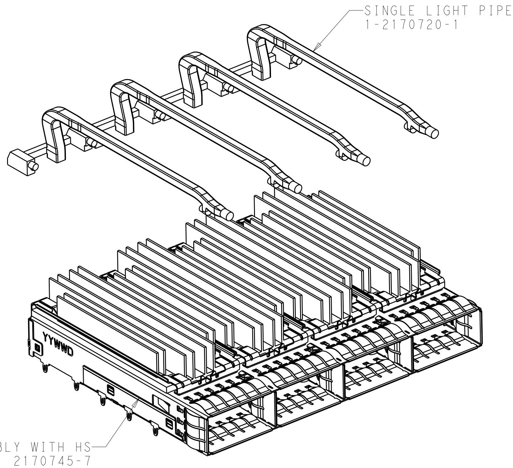
2170747-7 UNASSEMBLED 13 CAGE ASSY WITH HS AND LIGHT PIPE ARE UNASSEMBLED, AND PACKAGED INDIVIDUALLY. CUSTOMIZED HEAT SINK SCALE 2:1
