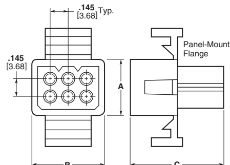
Plug
