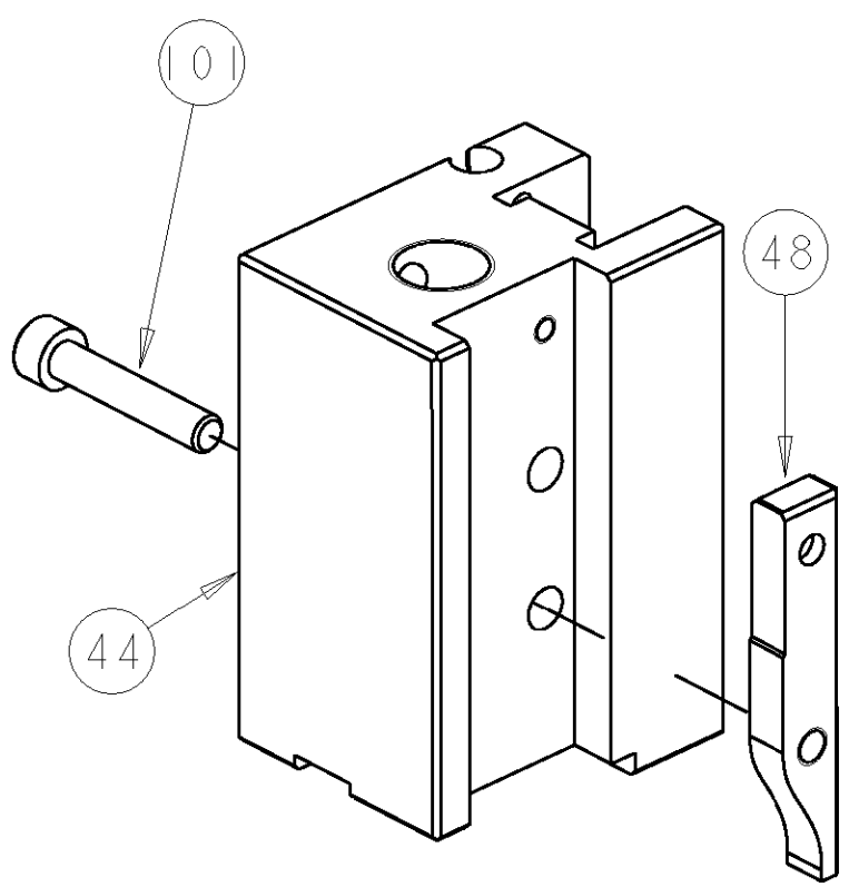
POST-FEED 1-5/8 STROKE
