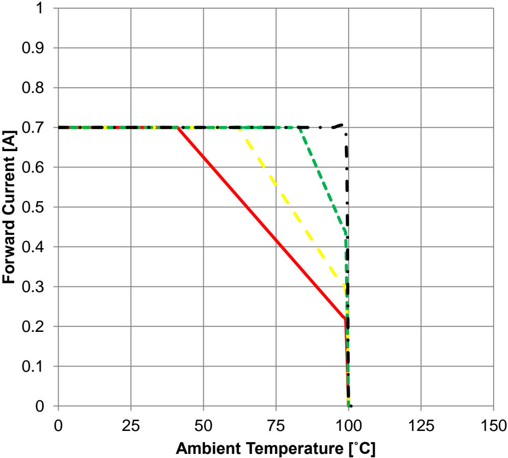
Derating Curve:
