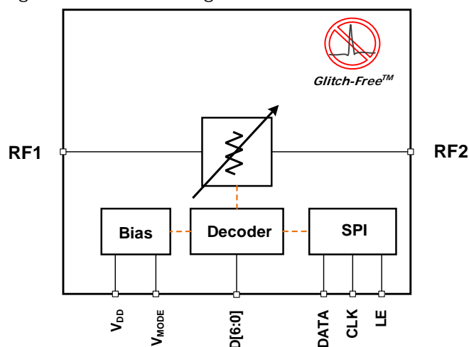
Figure 1. Block Diagram
