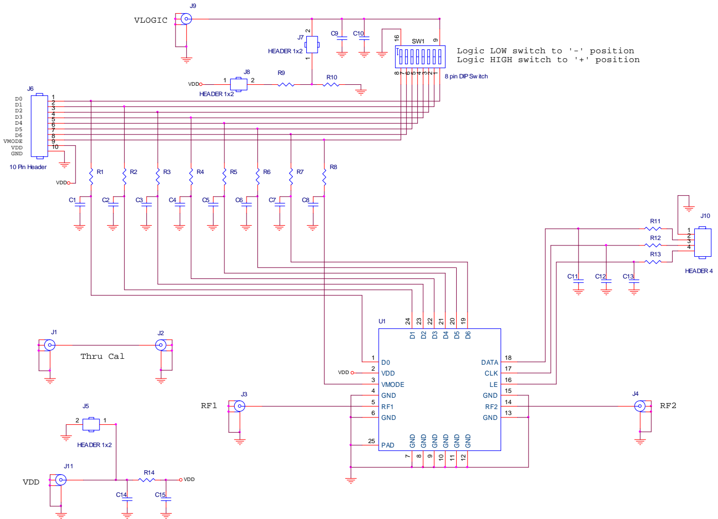
Figure 37. Electrical Schematic
