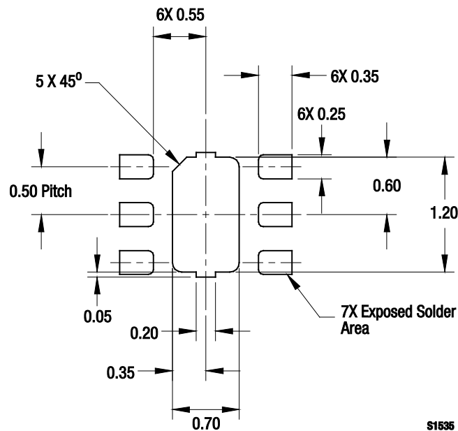
Figure 11. SKY13355-374LF PCB Layout Footprint (Top View)
