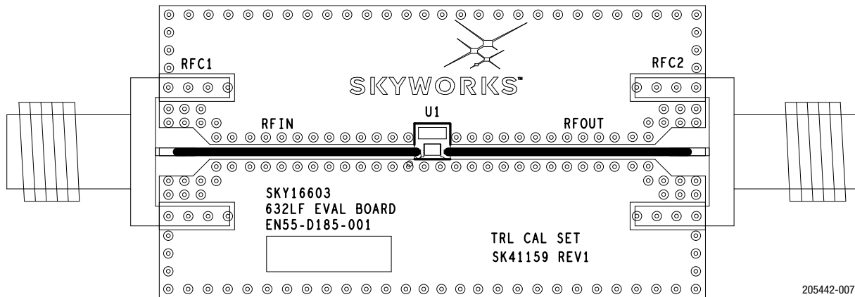
Figure 7. SKY16603-632LF Evaluation Board Assembly Diagram
