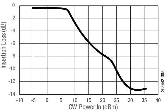
Figure 5. Insertion Loss vs CW Input Power In (f = 2.6 GHz)
