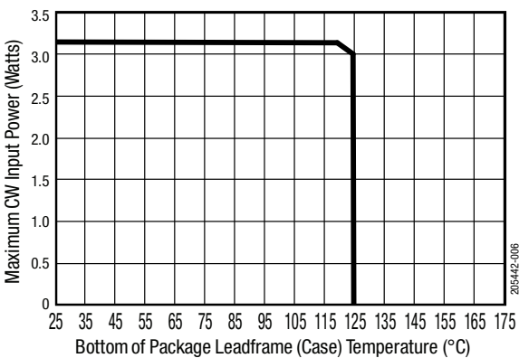
Figure 6. Power Derating Curve (Pd = 0.4 W @ 120°C) v Package Leadframe (Case) Temperature
