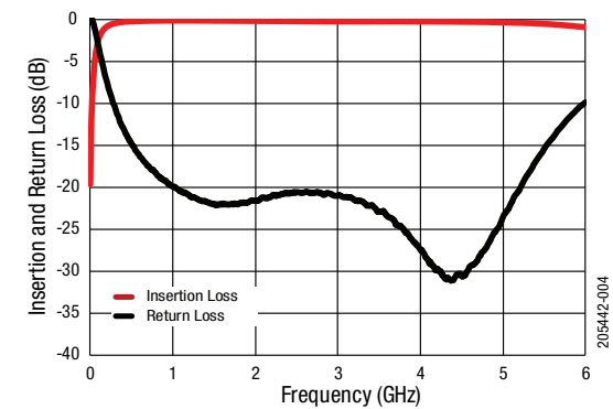
Figure 4. Small Signal Performance
