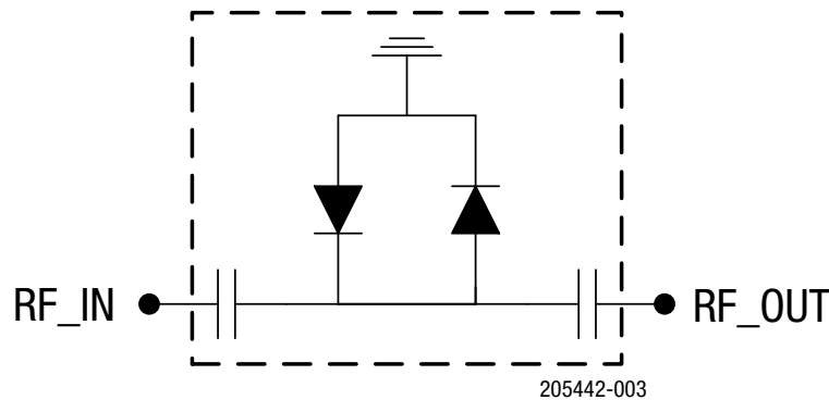
Figure 3. SKY16603-632LF Schematic
