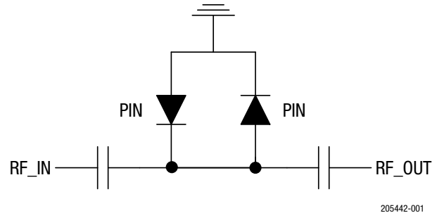
Figure 1. SKY16603-632LF Block Diagram
