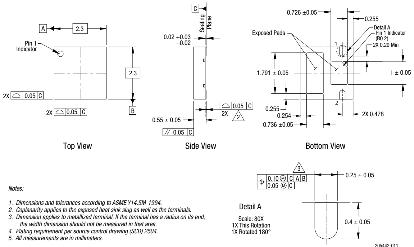
Figure 11. SKY16603-632LF Package Dimensions
