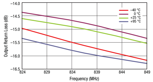
Figure 4. Output Return Loss vs Frequency Over Temperature
