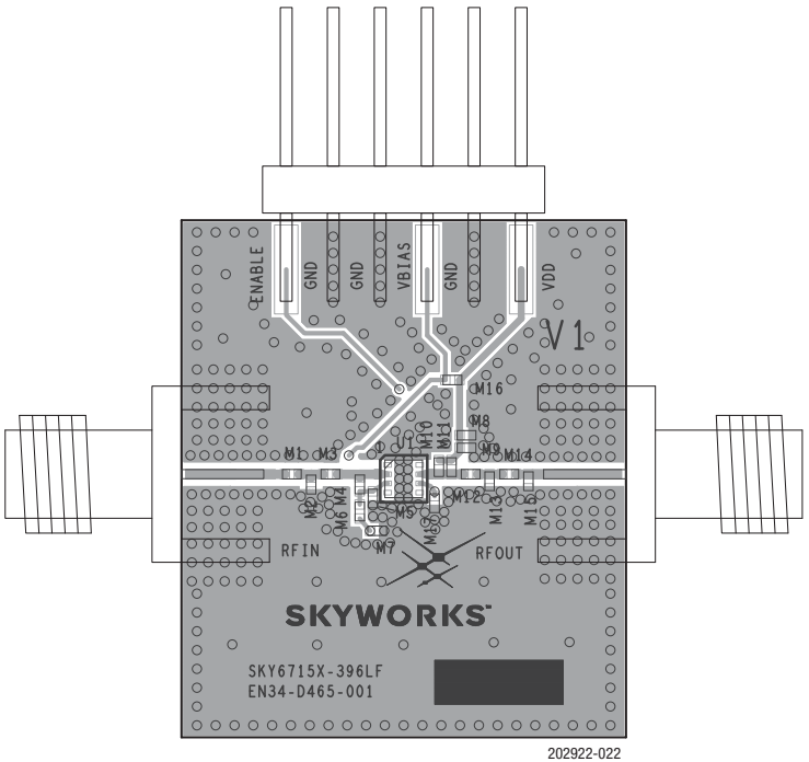
Figure 22. SKY67150-396LF Evaluation Board Assembly Diagram
