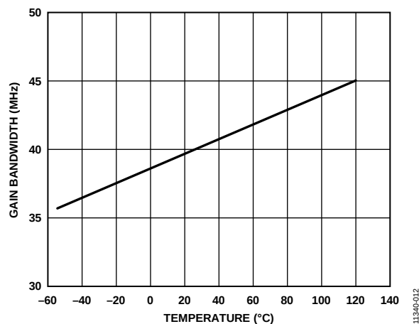
Figure 12. Gain Bandwidth Product vs. Temperature
