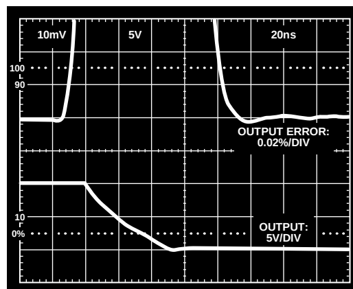
Figure 29. AD841 0.01% Settling Time
