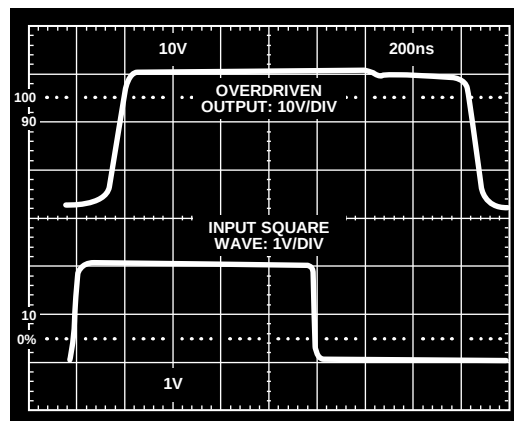
Figure 34. Overdrive Recovery
