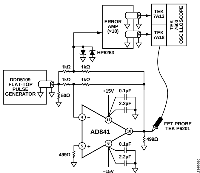
Figure 30. Settling Time Test Circuit
