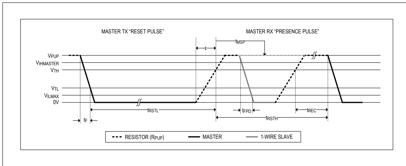
Figure 4. 1-Wire Reset/Presence-Detect Cycle
