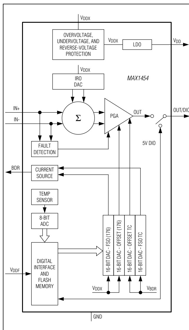
Figure 1. Functional Diagram
