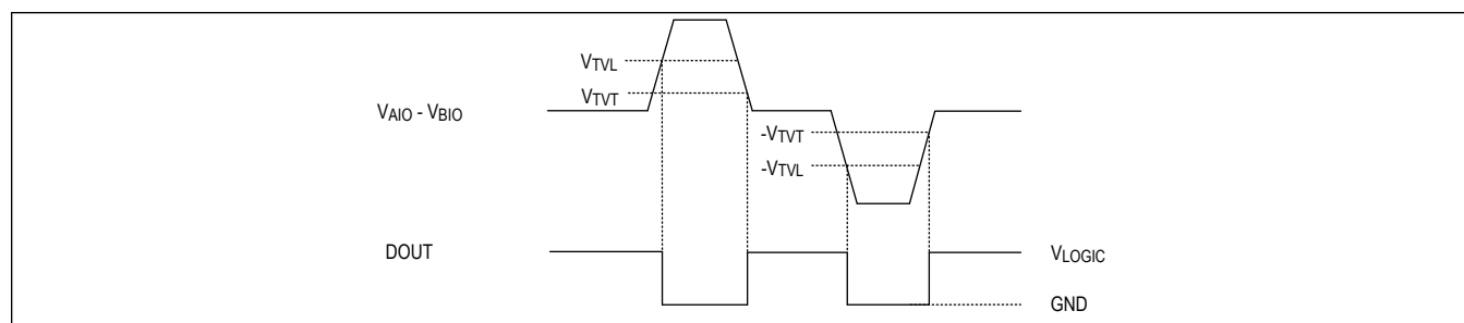
Figure 6. Receiver Thresholds
