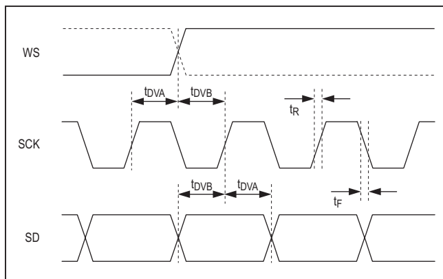
Figure 15. Output I²S Timing Parameters
