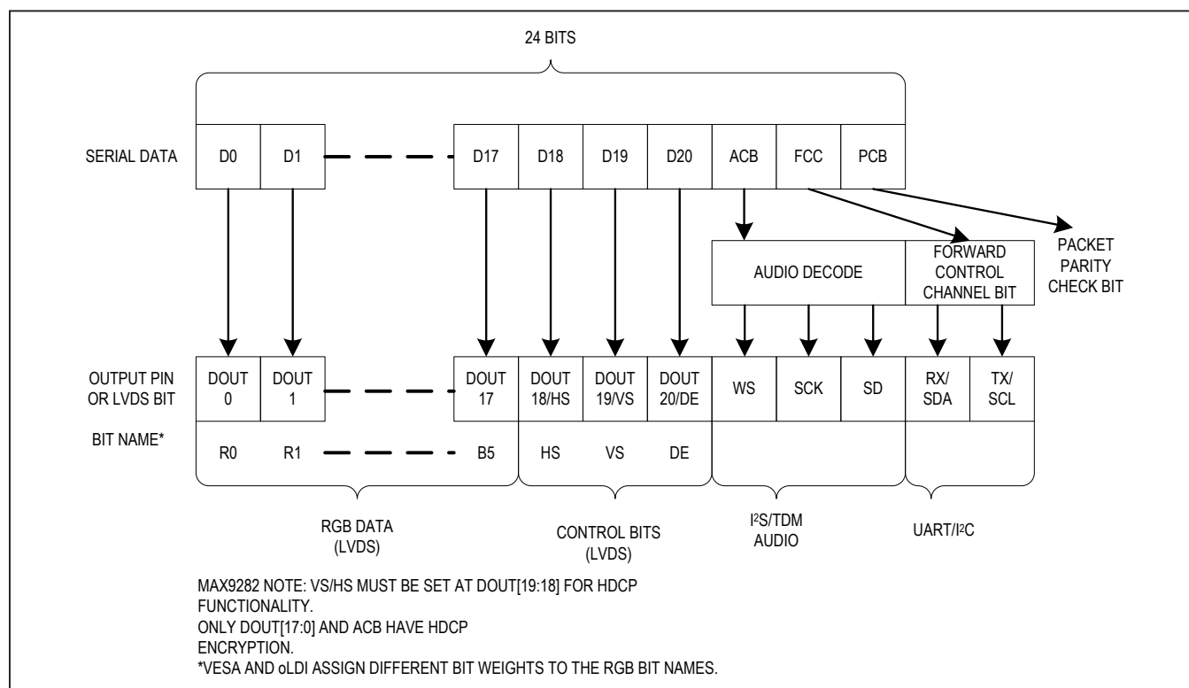
Figure 17. LVDS Clock and Bit Assignment
