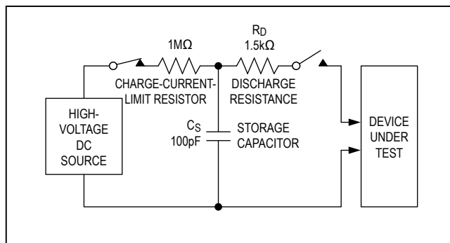
Figure 26. Human Body Model ESD Test Circuit
