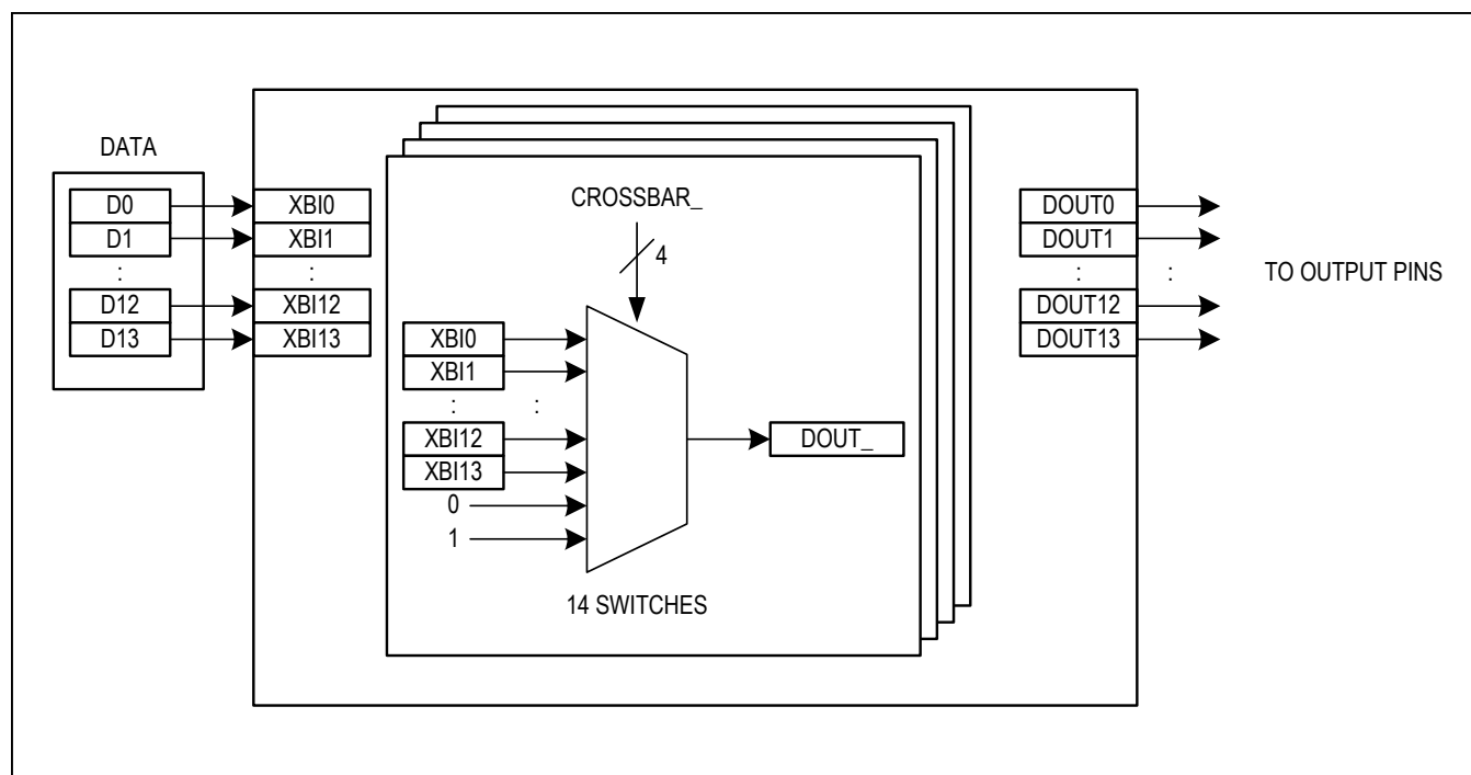
Figure 18. Crosspoint-Switch Dataflow
