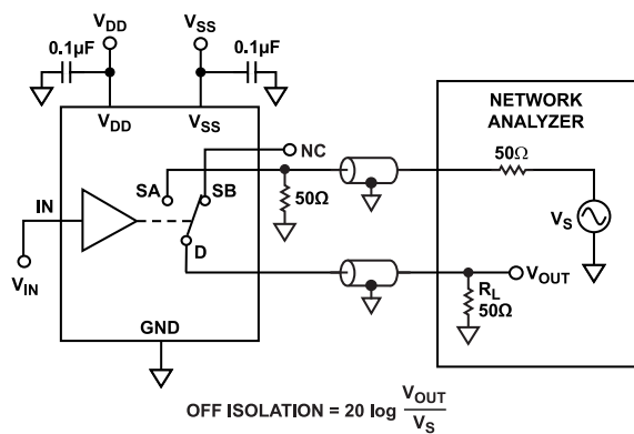
Figure 25. Off Isolation
