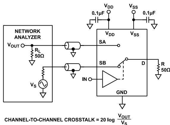
Figure 26. Channel-to-Channel Crosstalk
