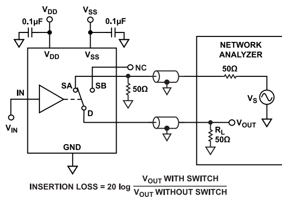
Figure 27. Bandwidth
