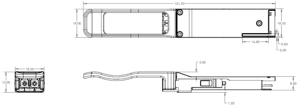
Figure 2 – FTL4C2QE1C mechanical drawing
