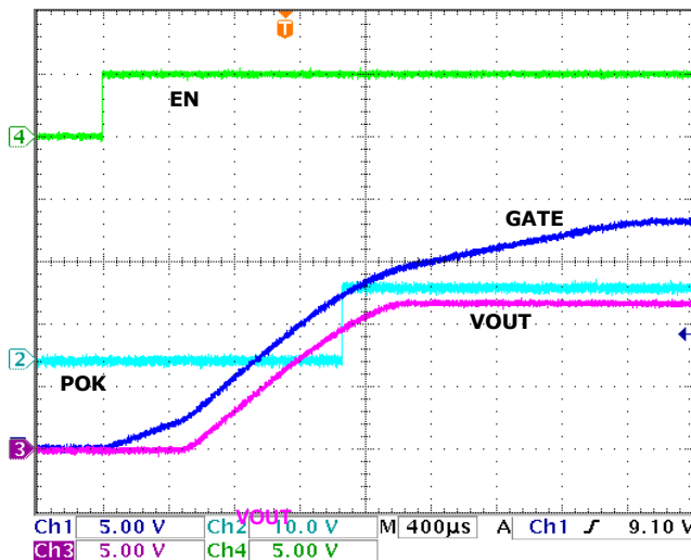
FIGURE 10. ES1010SI TURN-ON
