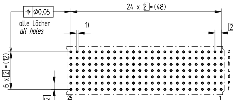
Board hole pattern (Component mounting side)
