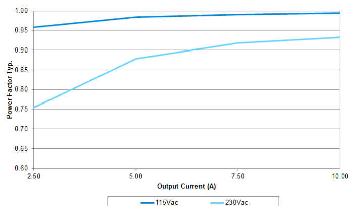
Fig. 4 Power Factor VS Output Load at 24V
