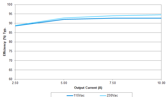
Fig. 2 Efficiency VS Output Load at 24V
